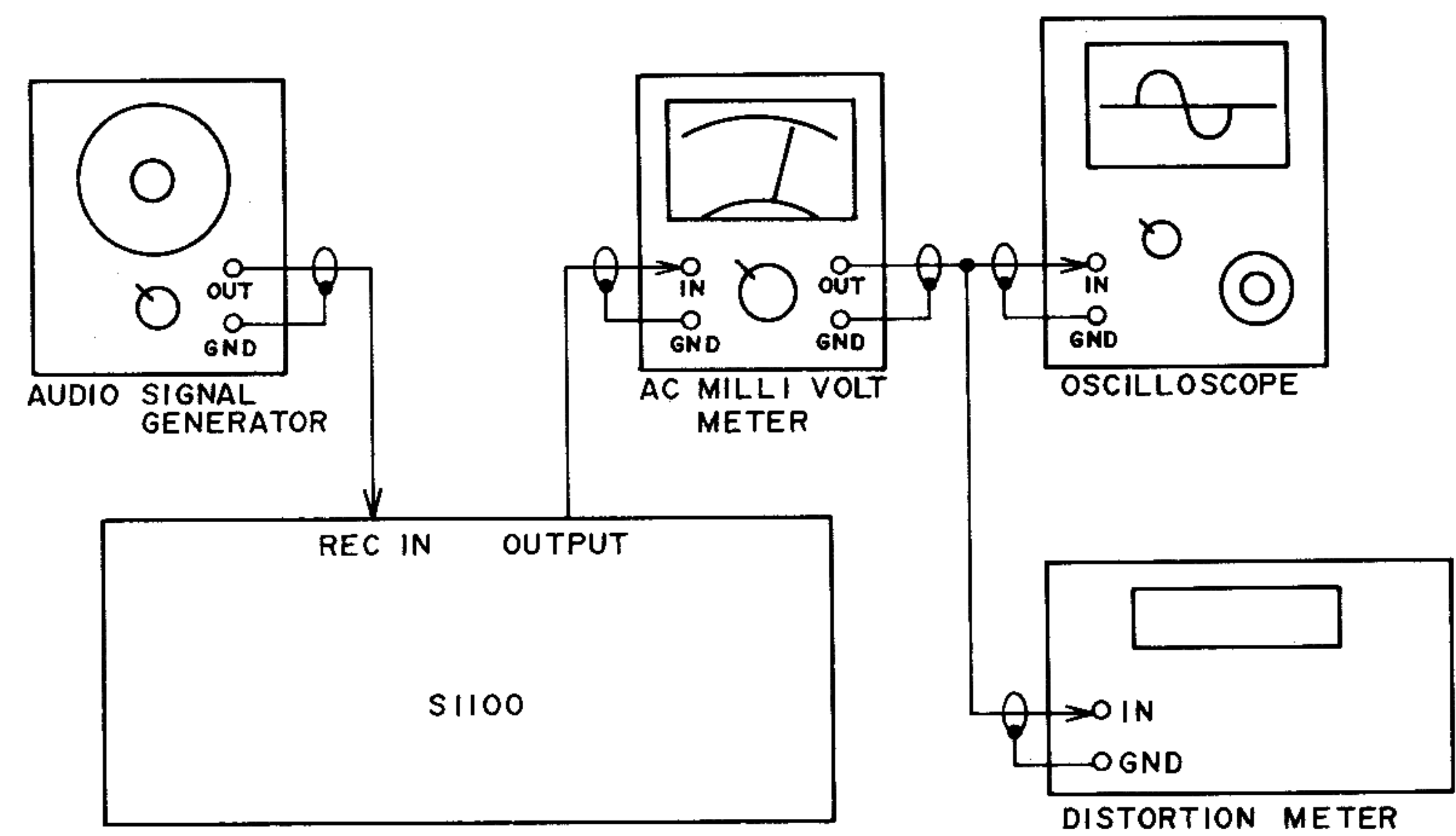
Fig. 3-1 Instrument connection
